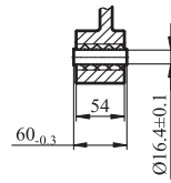
GSH/GSHZ/GSHF77输出轴
