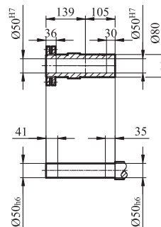
GSH/GSHZ/GSHF77输出轴
